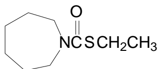
Figure 1. Chemical structure of molinate
